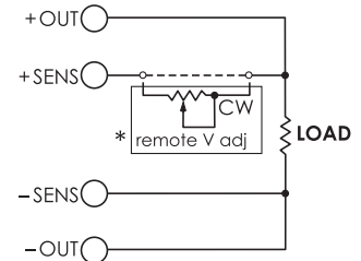
Output Connections when Remote Sensing Option is included:
